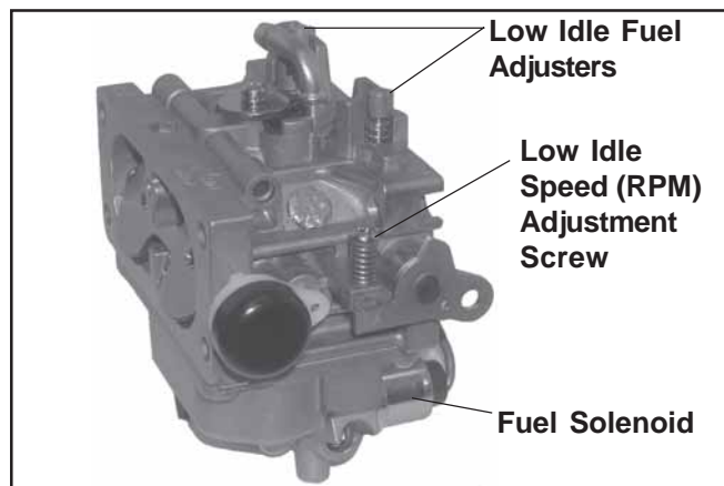
Figure 22. Keihin Two-Barrel Carburetor.
