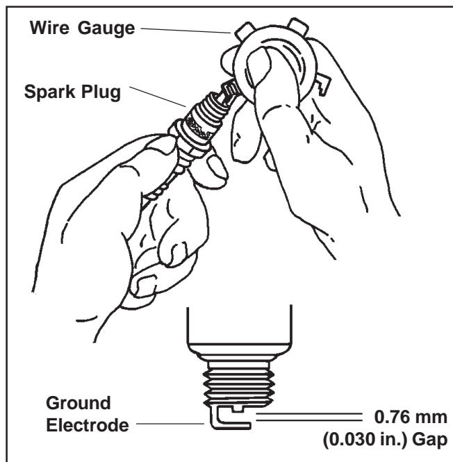
Figure 16. Servicing Spark Plug.
