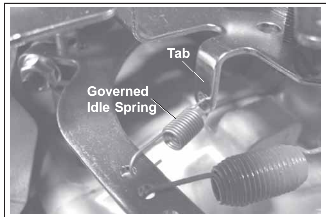
Figure 20. Governed Idle Spring Location.
