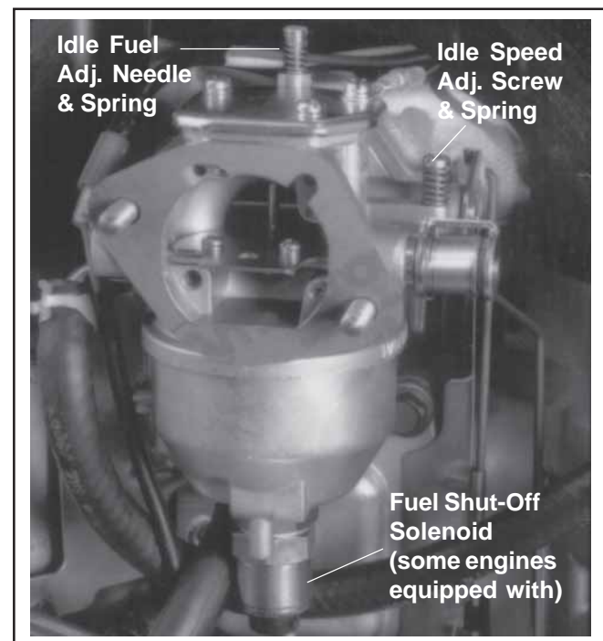
Figure 19. Carburetor CV18-23, CV620-CV730, CV740.
