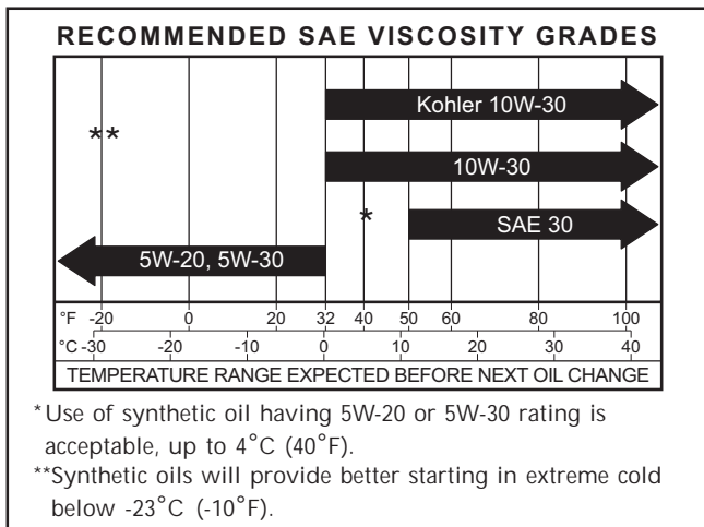
Figure 2. Viscosity Grades Table.
