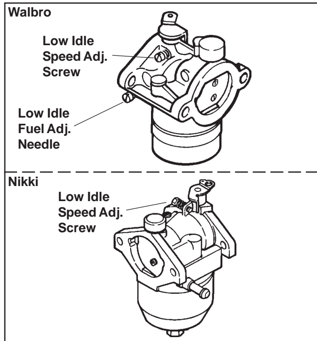
Figure 11. Carburetor.
